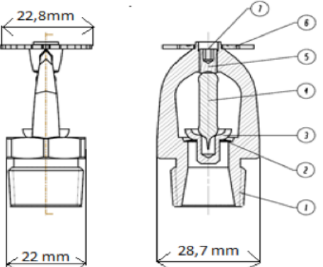
Pendent
