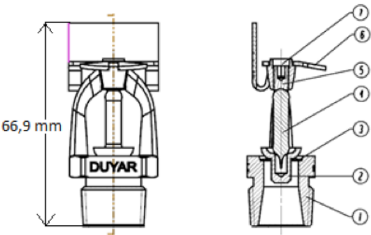
Sidewall
